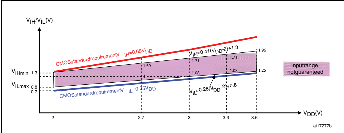
Figure 22. Standard I/O input characteristics - CMOS port
