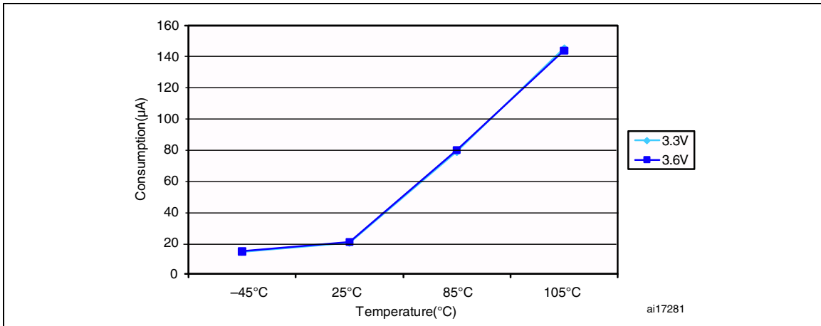
Figure 15. Typical current consumption in Stop mode with regulator in Run mode versus temperature at V_{DD} = 3.3\text{ V} and 3.6\text{ V}
